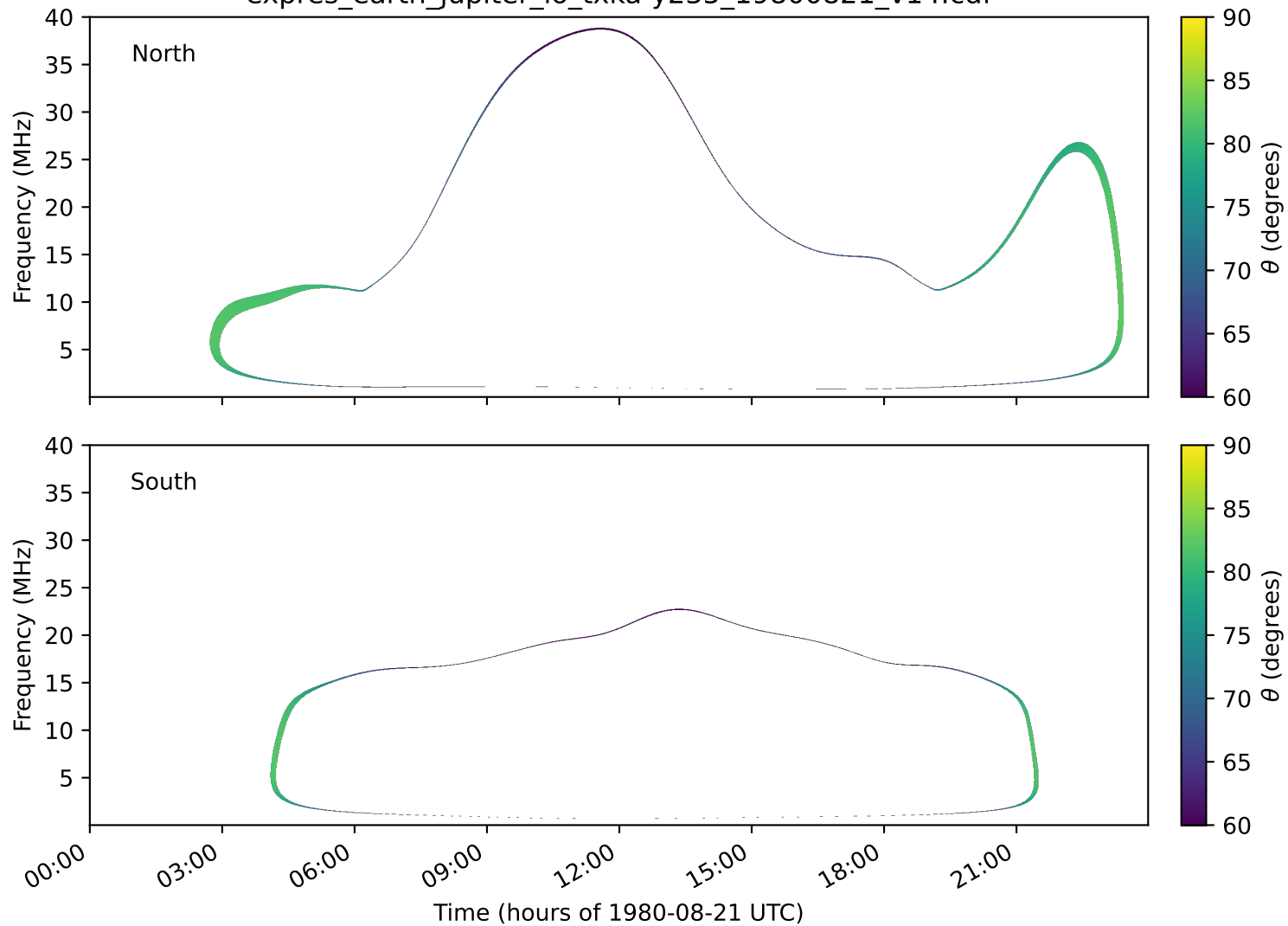
expres_earth_jupiter_io_txka-y235_19800821_v14.cdf
