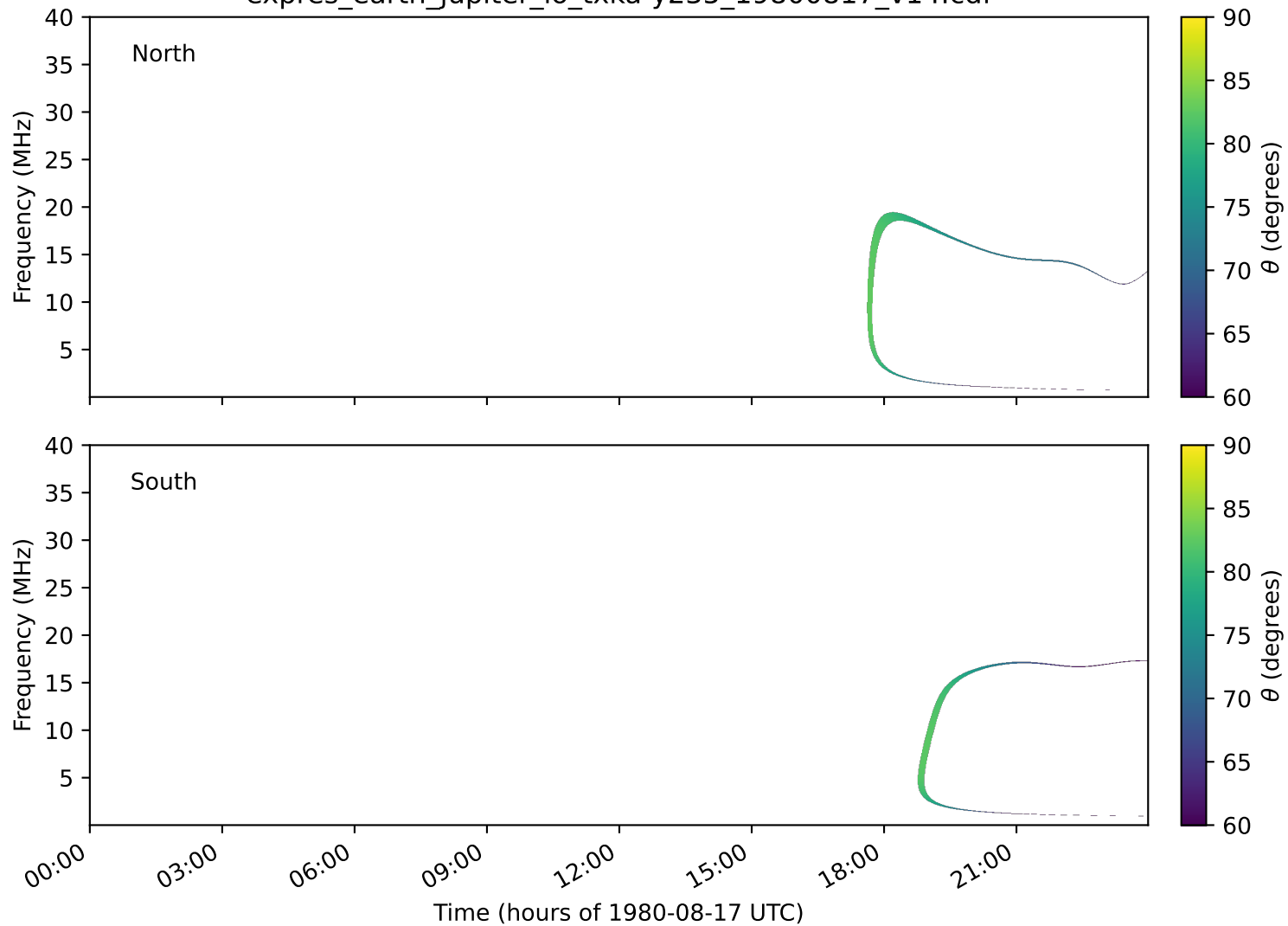
expres_earth_jupiter_io_txka-y235_19800817_v14.cdf
