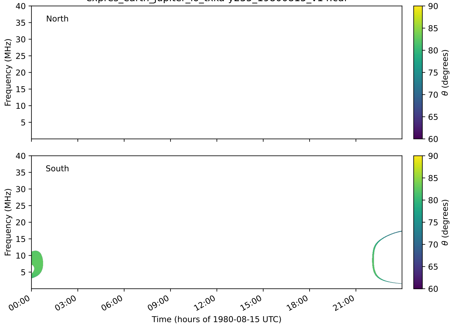
expres_earth_jupiter_io_txka-y235_19800815_v14.cdf
