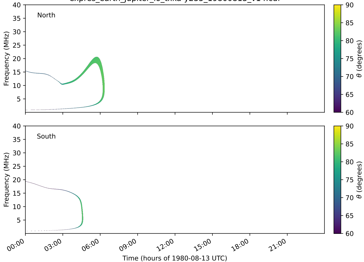
expres_earth_jupiter_io_txka-y235_19800813_v14.cdf
