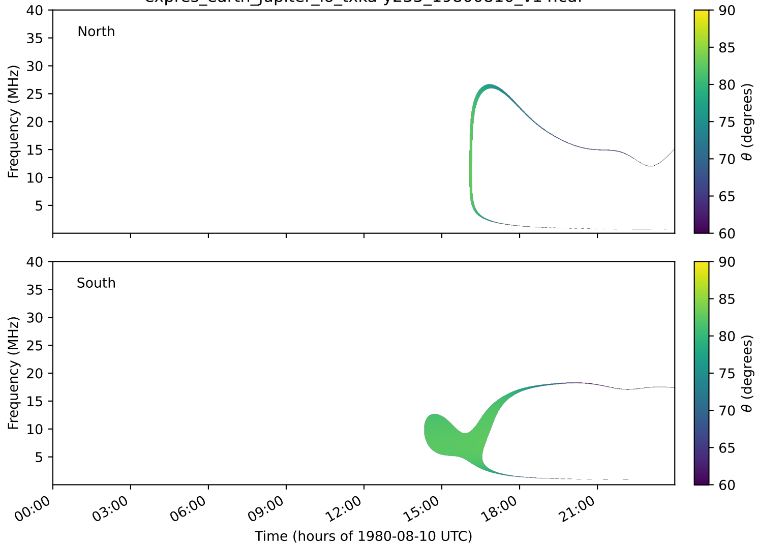
expres_earth_jupiter_io_txka-y235_19800810_v14.cdf
