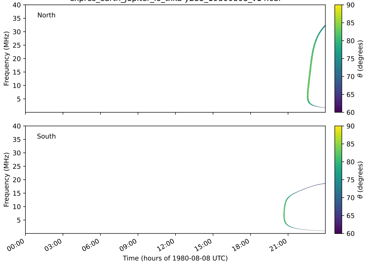
expres_earth_jupiter_io_txka-y235_19800808_v14.cdf
