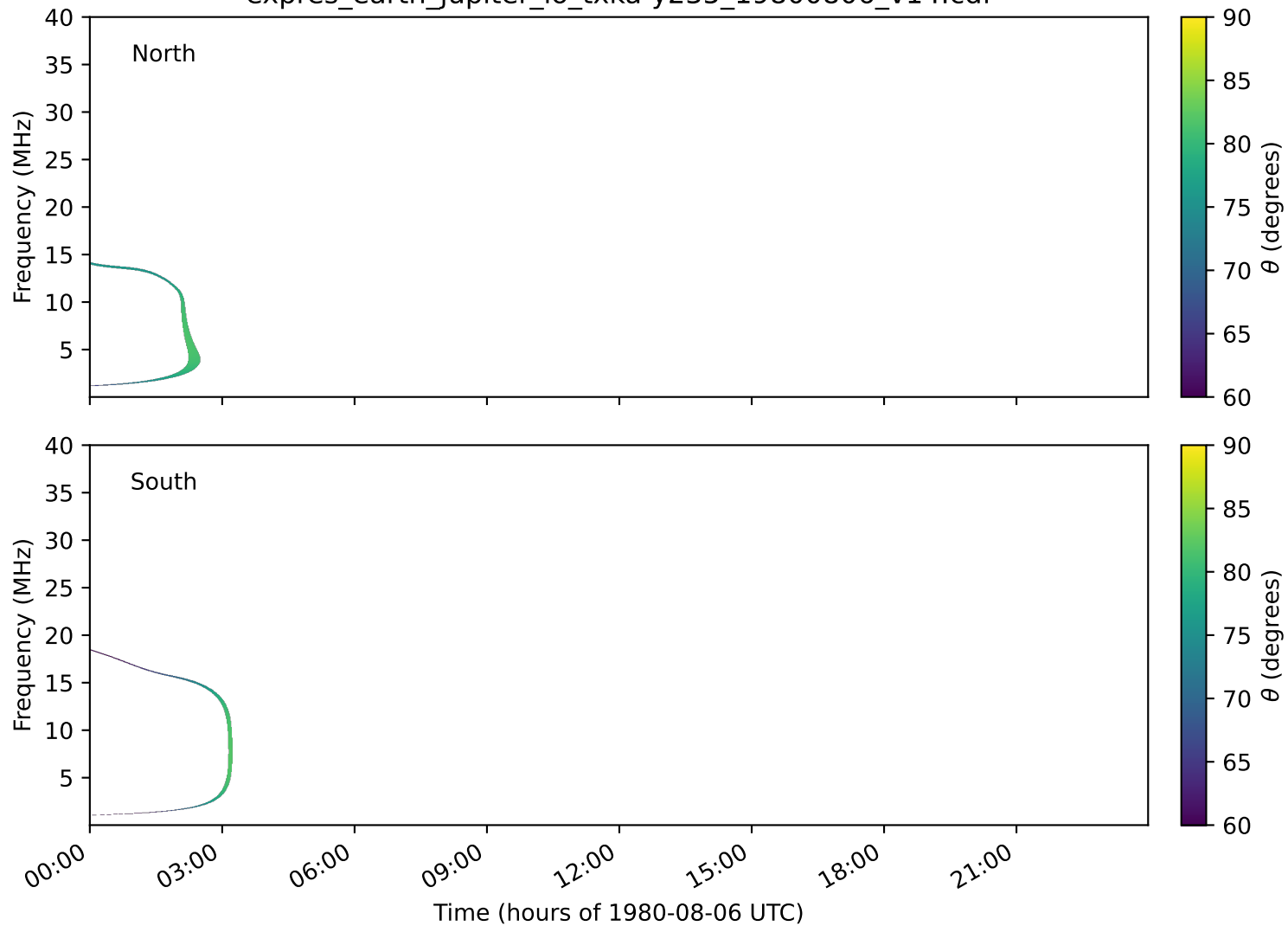
expres_earth_jupiter_io_txka-y235_19800806_v14.cdf
