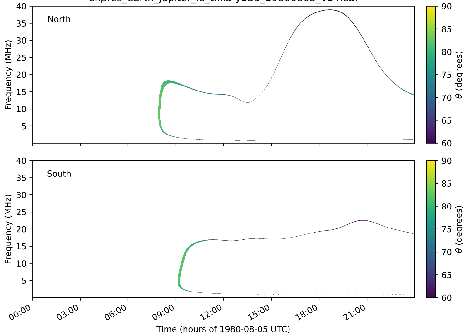
expres_earth_jupiter_io_txka-y235_19800805_v14.cdf
