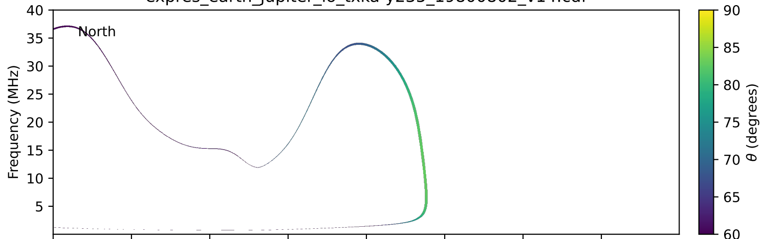
expres_earth_jupiter_io_txka-y235_19800802_v14.cdf
