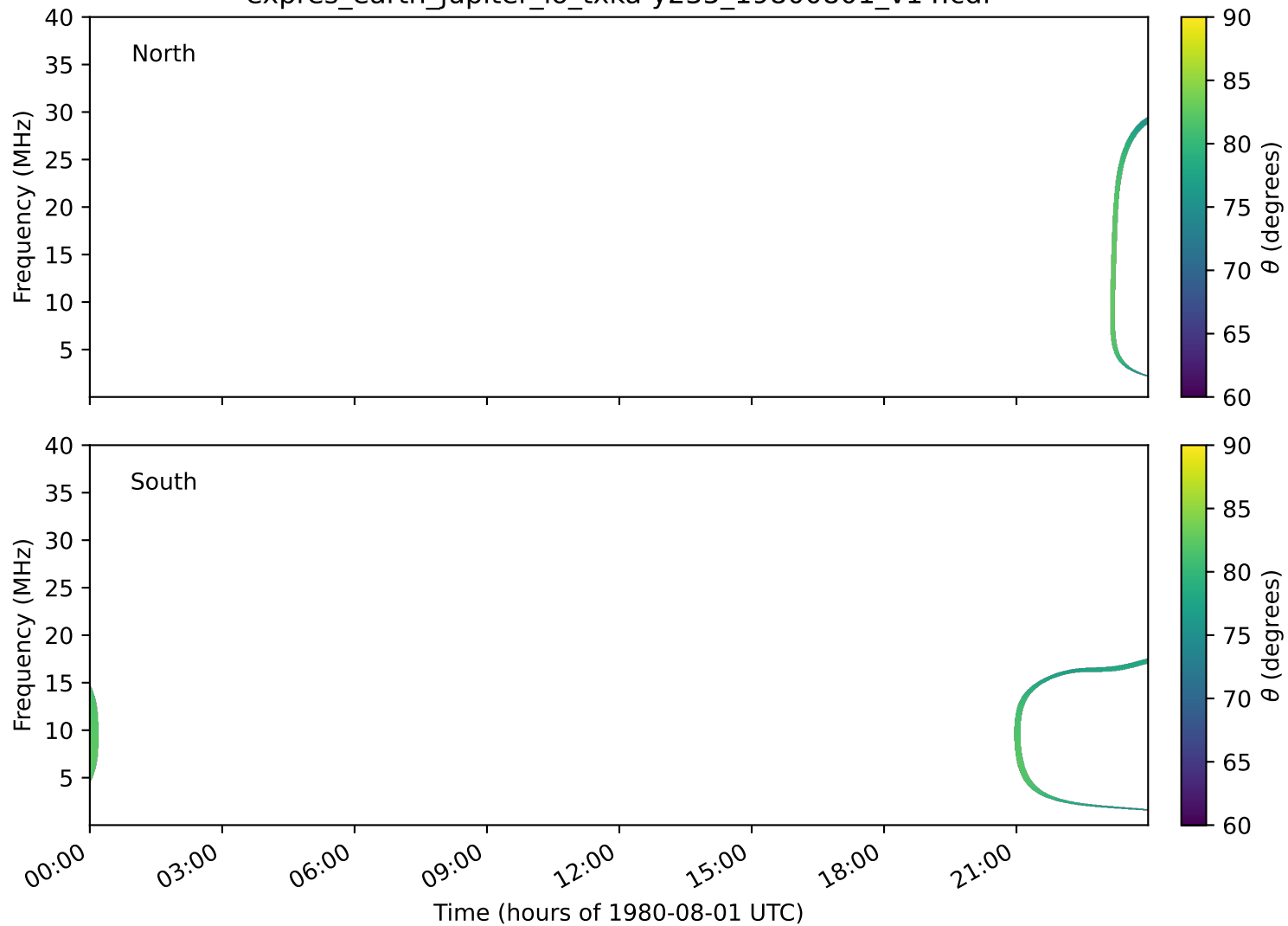
expres_earth_jupiter_io_txka-y235_19800801_v14.cdf
