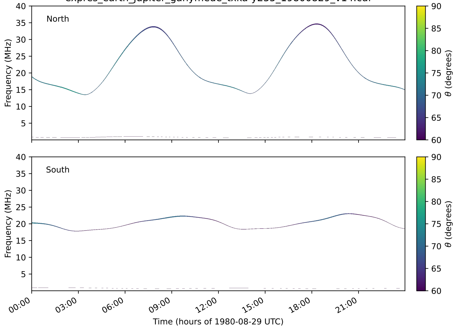
expres_earth_jupiter_ganymede_txka-y235_19800829_v14.cdf
