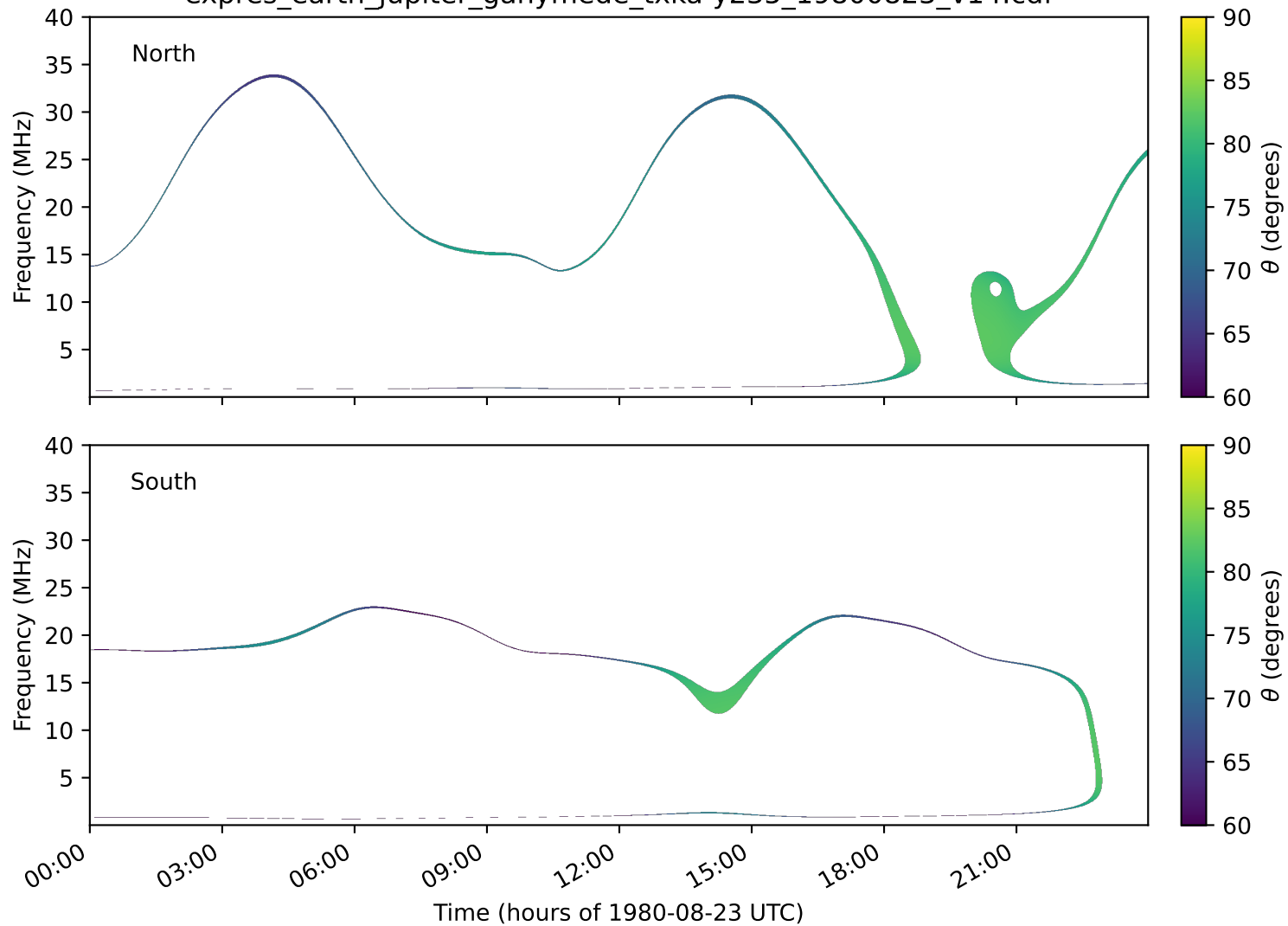
expres_earth_jupiter_ganymede_txka-y235_19800823_v14.cdf
