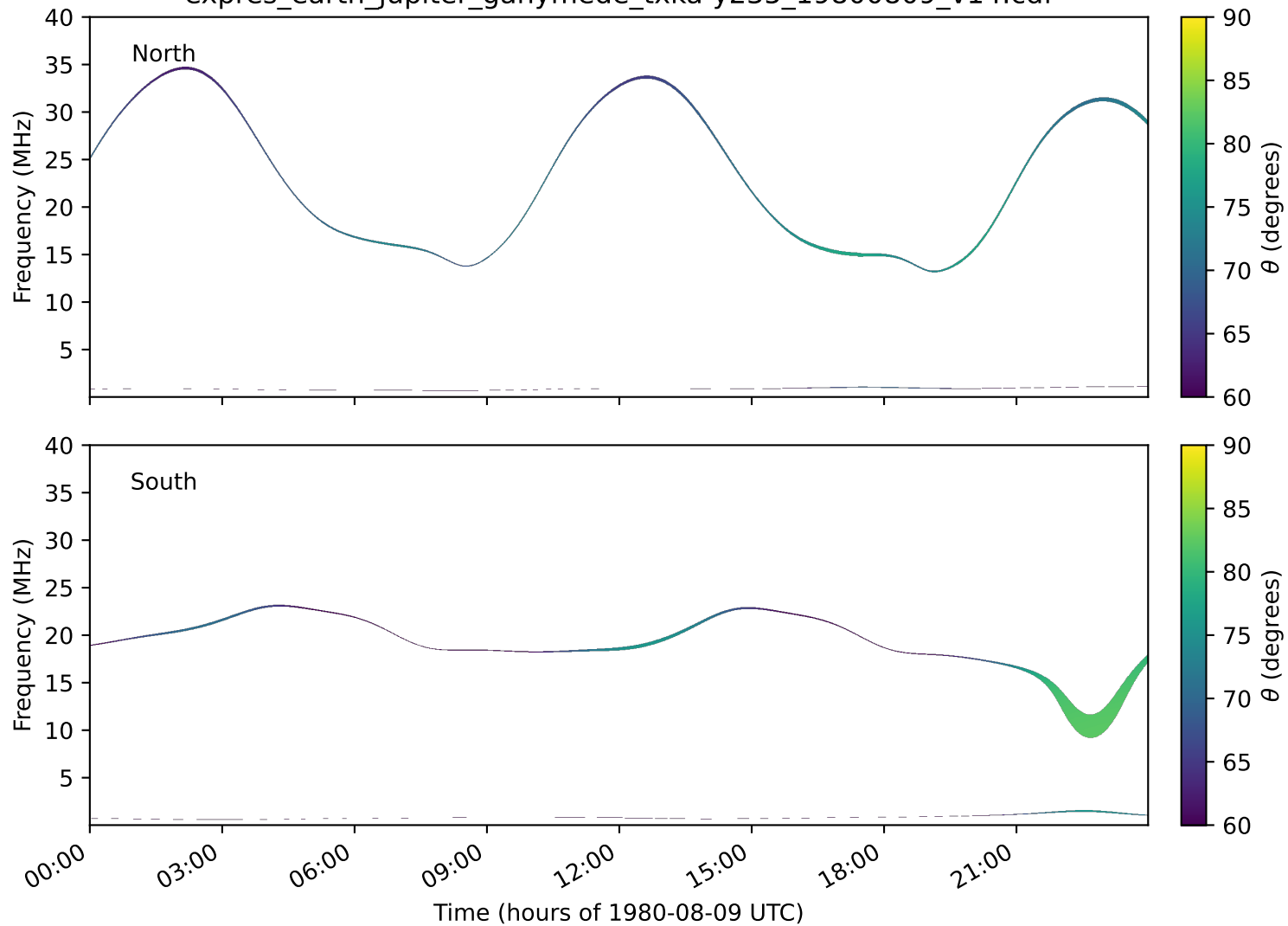
expres_earth_jupiter_ganymede_txka-y235_19800809_v14.cdf
