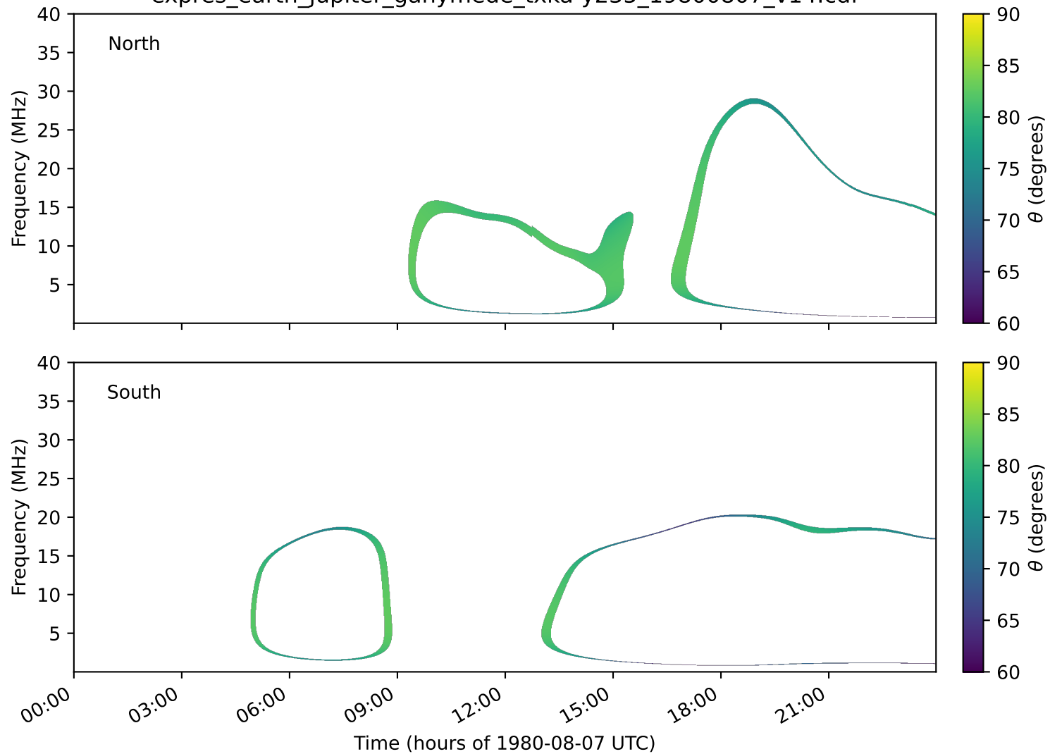
expres_earth_jupiter_ganymede_txka-y235_19800807_v14.cdf
