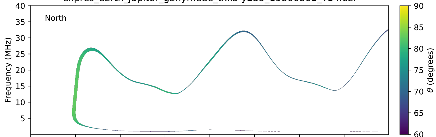
expres_earth_jupiter_ganymede_txka-y235_19800801_v14.cdf
