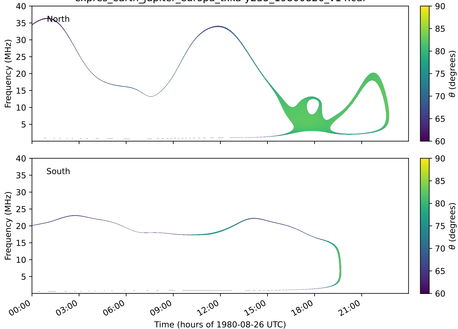
expres_earth_jupiter_europa_txka-y235_19800826_v14.cdf
