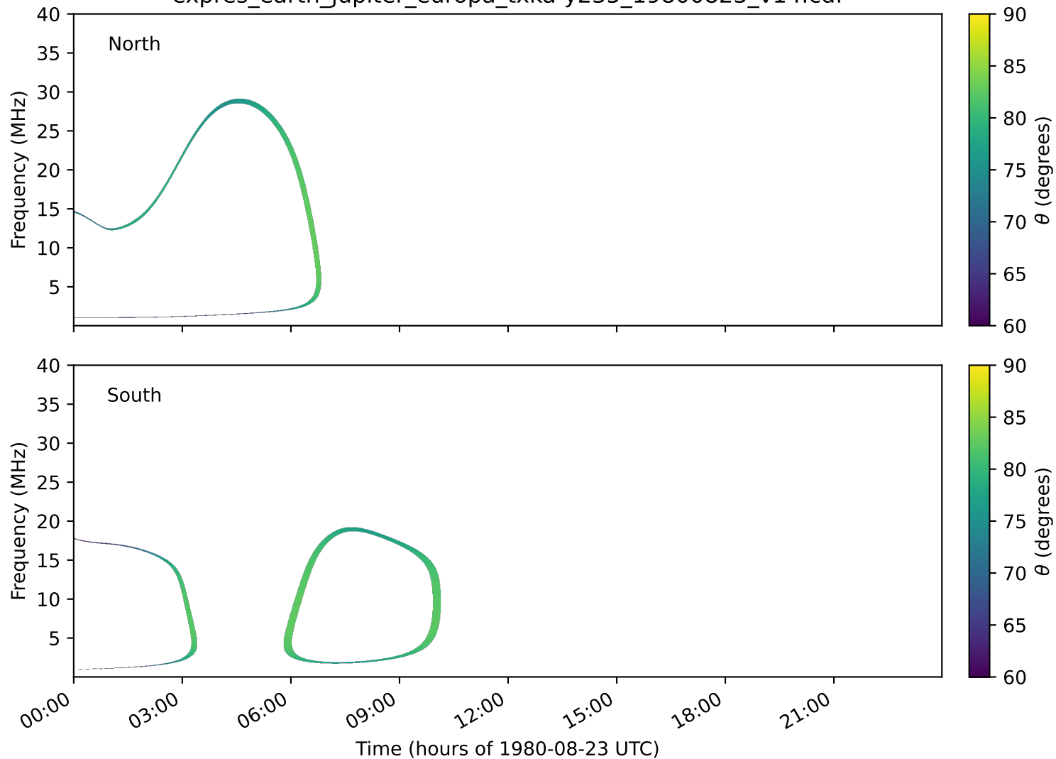
expres_earth_jupiter_europa_txka-y235_19800823_v14.cdf
