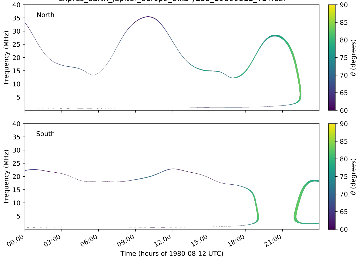
expres_earth_jupiter_europa_txka-y235_19800812_v14.cdf
