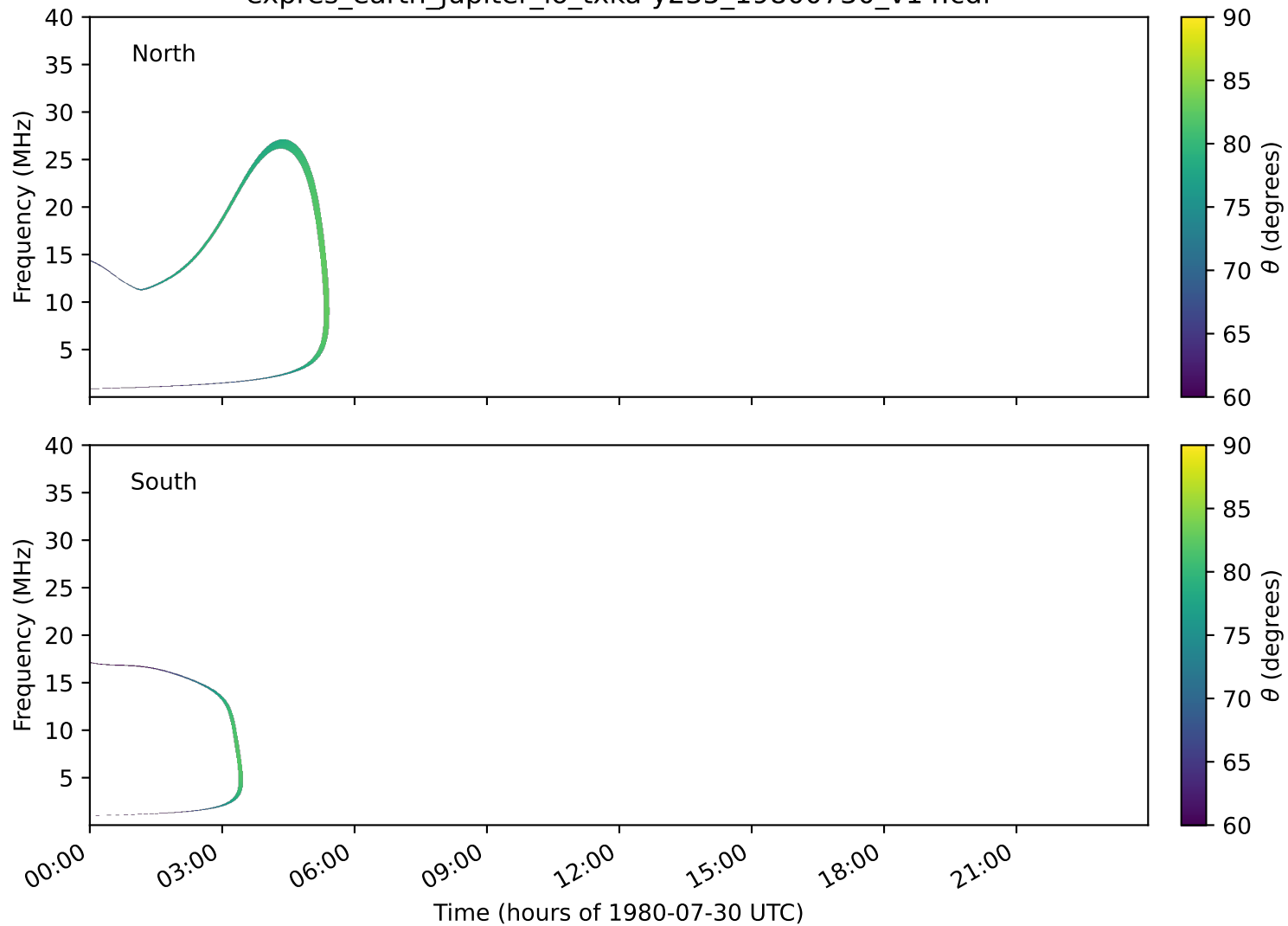
expres_earth_jupiter_io_txka-y235_19800730_v14.cdf
