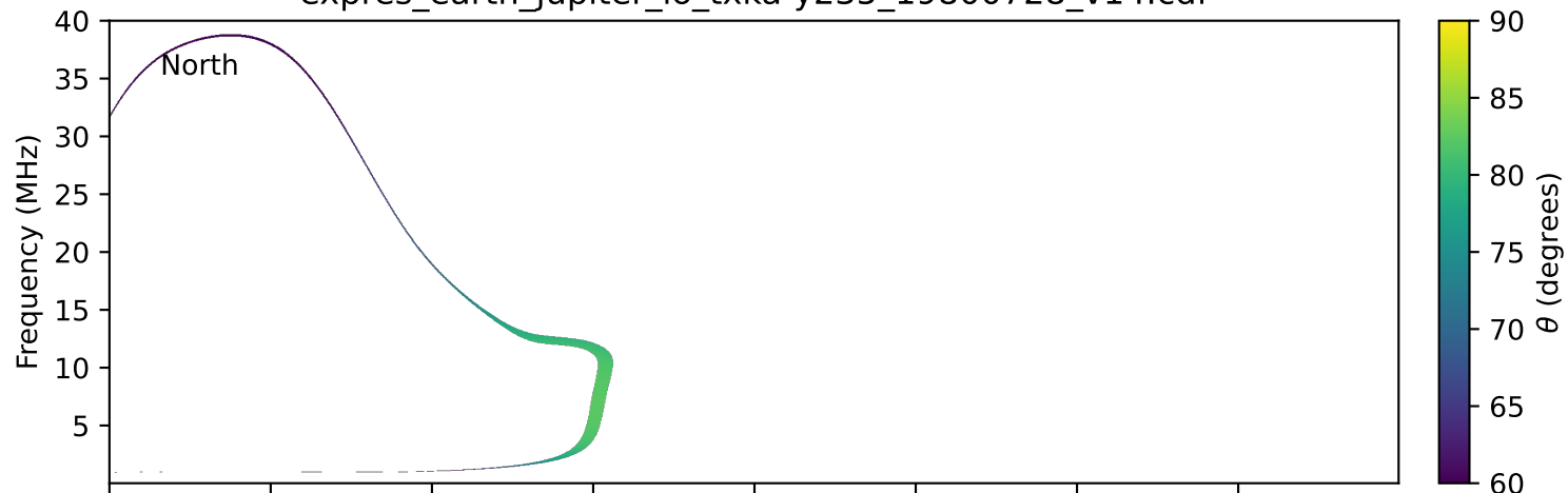
expres_earth_jupiter_io_txka-y235_19800728_v14.cdf
