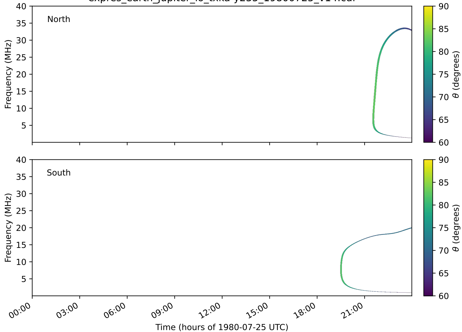
expres_earth_jupiter_io_txka-y235_19800725_v14.cdf
