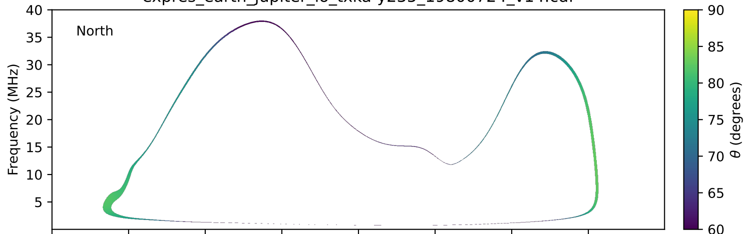
expres_earth_jupiter_io_txka-y235_19800724_v14.cdf
