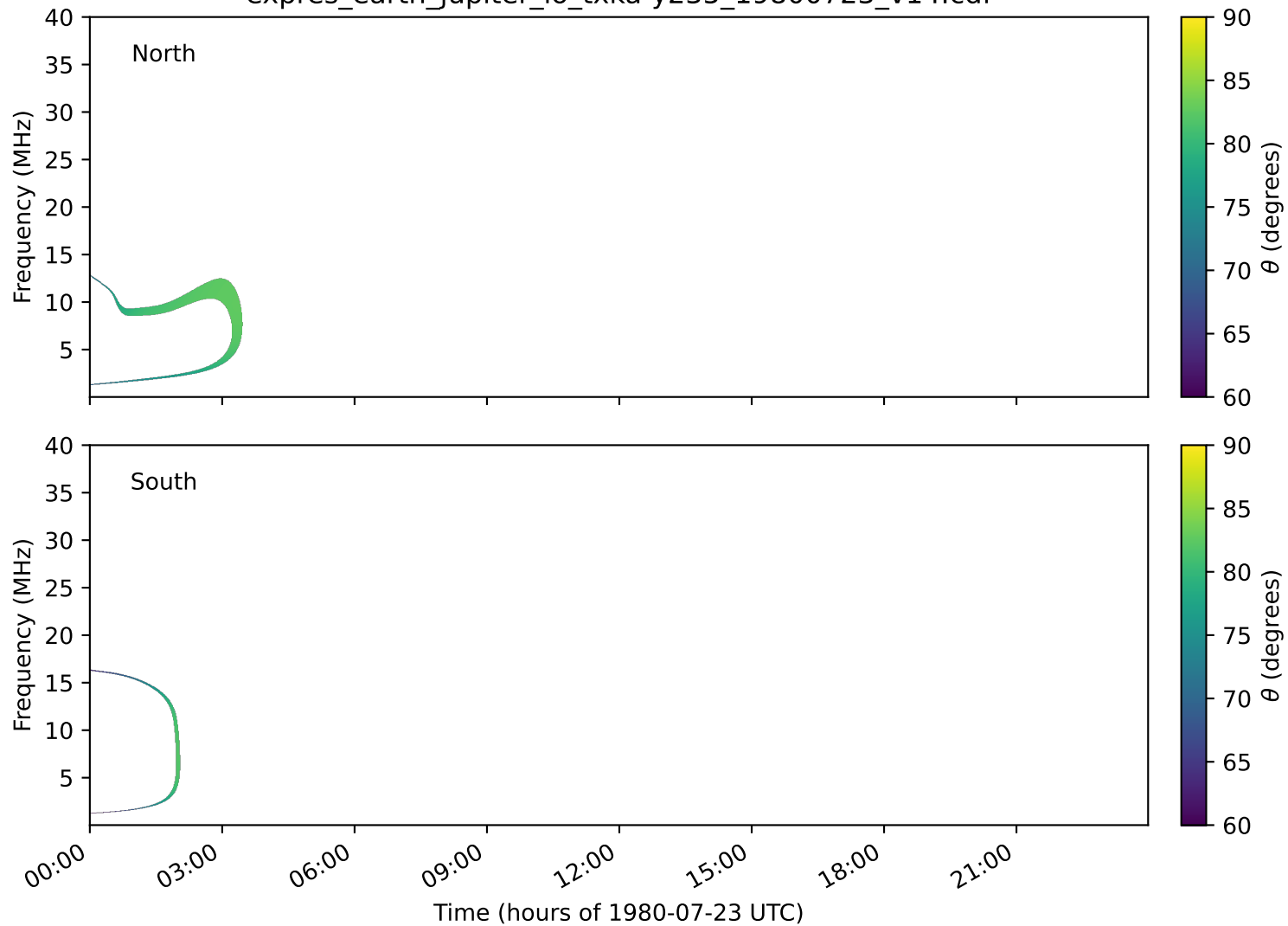
expres_earth_jupiter_io_txka-y235_19800723_v14.cdf
