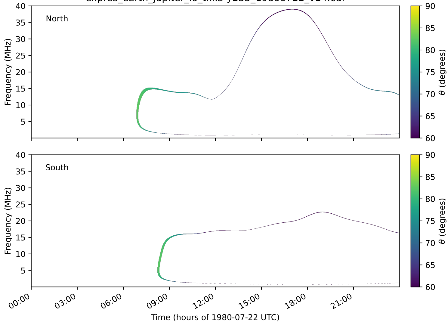
expres_earth_jupiter_io_txka-y235_19800722_v14.cdf
