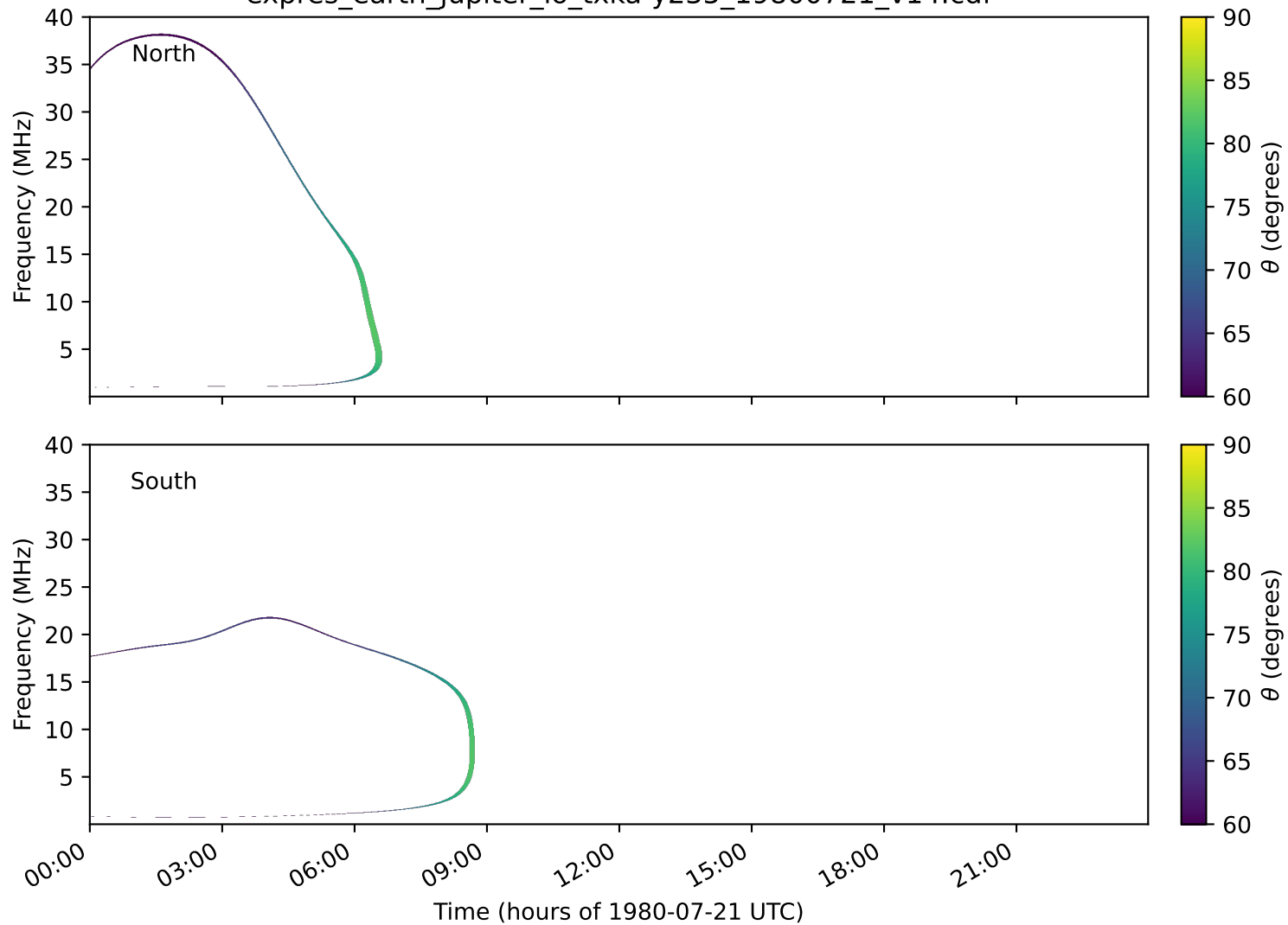
expres_earth_jupiter_io_txka-y235_19800721_v14.cdf
