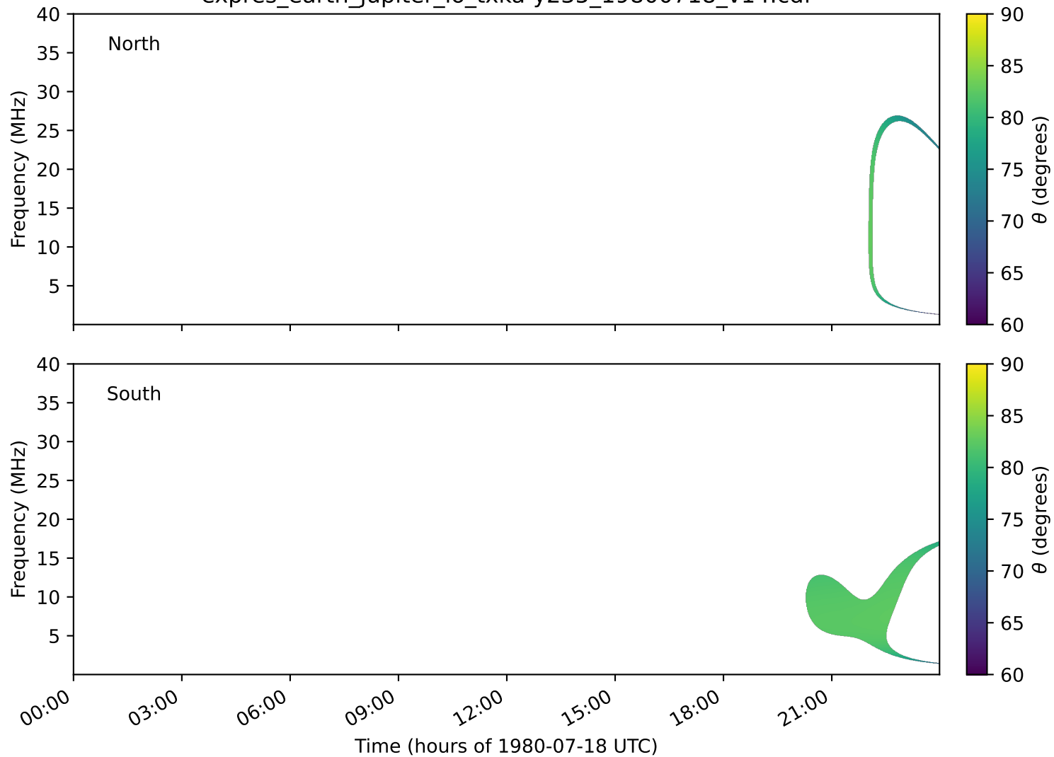
expres_earth_jupiter_io_txka-y235_19800718_v14.cdf
