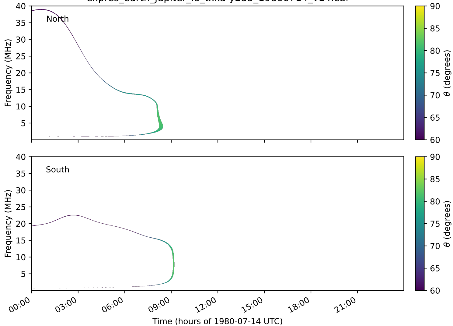
expres_earth_jupiter_io_txka-y235_19800714_v14.cdf
