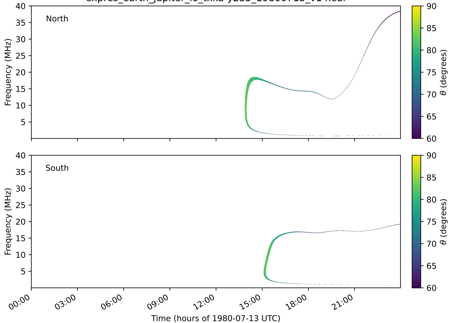
expres_earth_jupiter_io_txka-y235_19800713_v14.cdf
