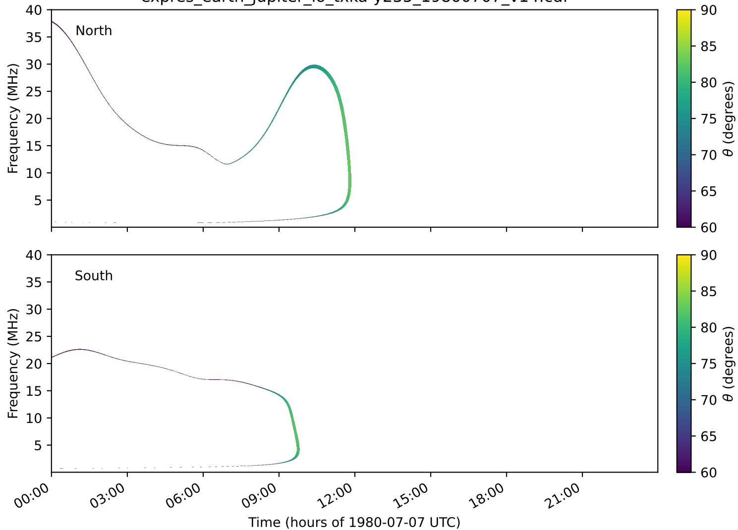
expres_earth_jupiter_io_txka-y235_19800707_v14.cdf
