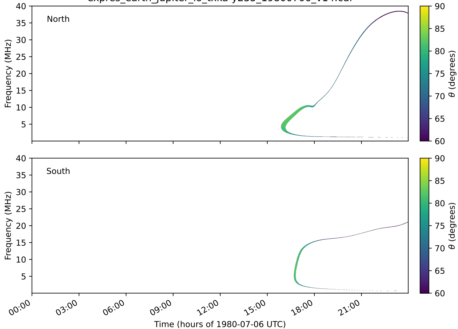
expres_earth_jupiter_io_txka-y235_19800706_v14.cdf
