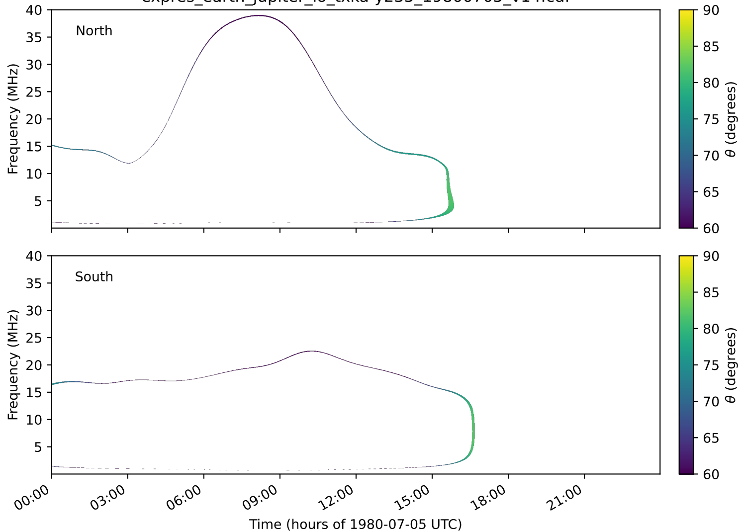
expres_earth_jupiter_io_txka-y235_19800705_v14.cdf
