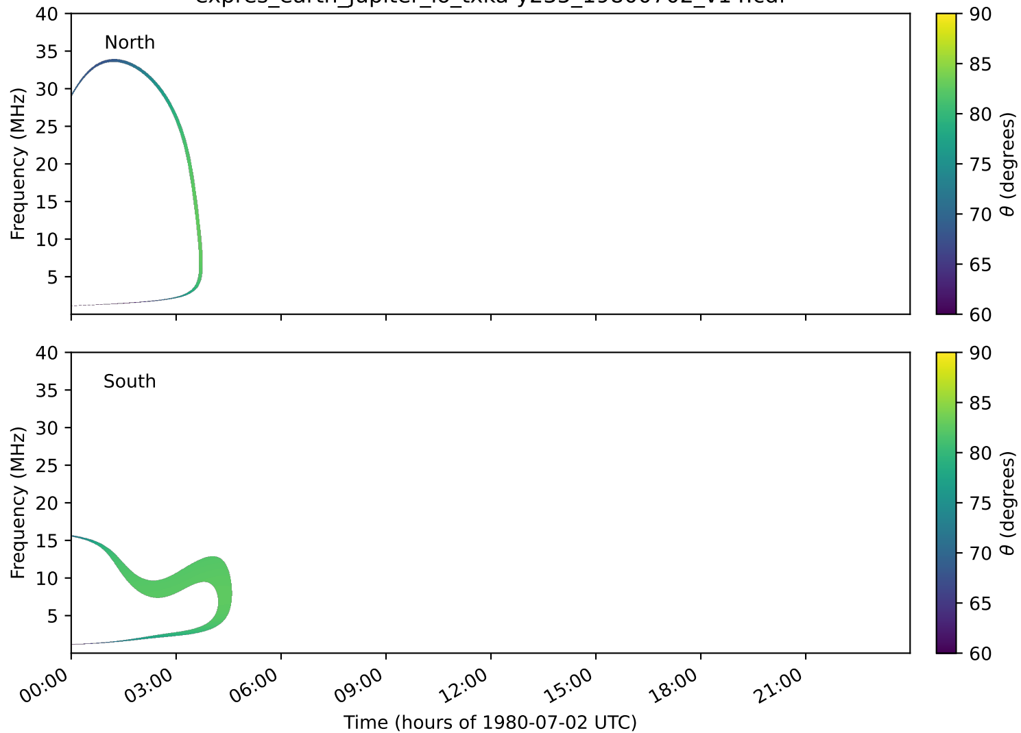
expres_earth_jupiter_io_txka-y235_19800702_v14.cdf
