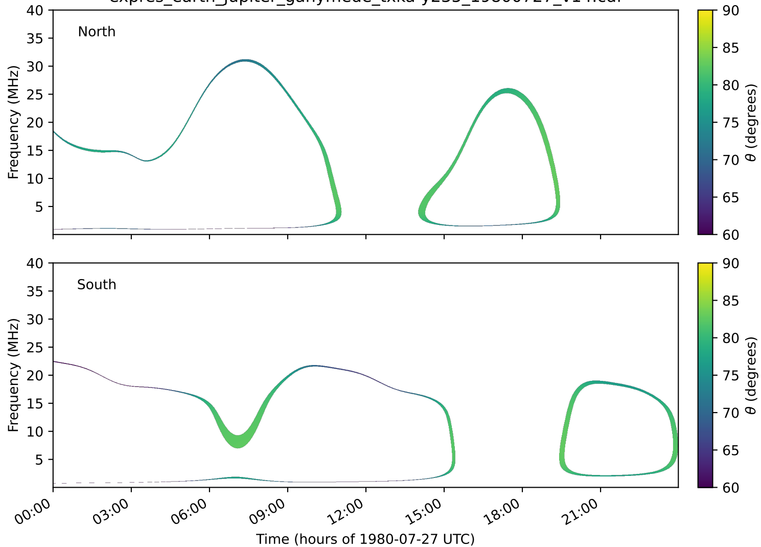
expres_earth_jupiter_ganymede_txka-y235_19800727_v14.cdf
