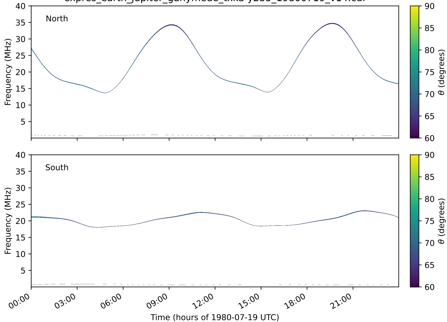
expres_earth_jupiter_ganymede_txka-y235_19800719_v14.cdf
