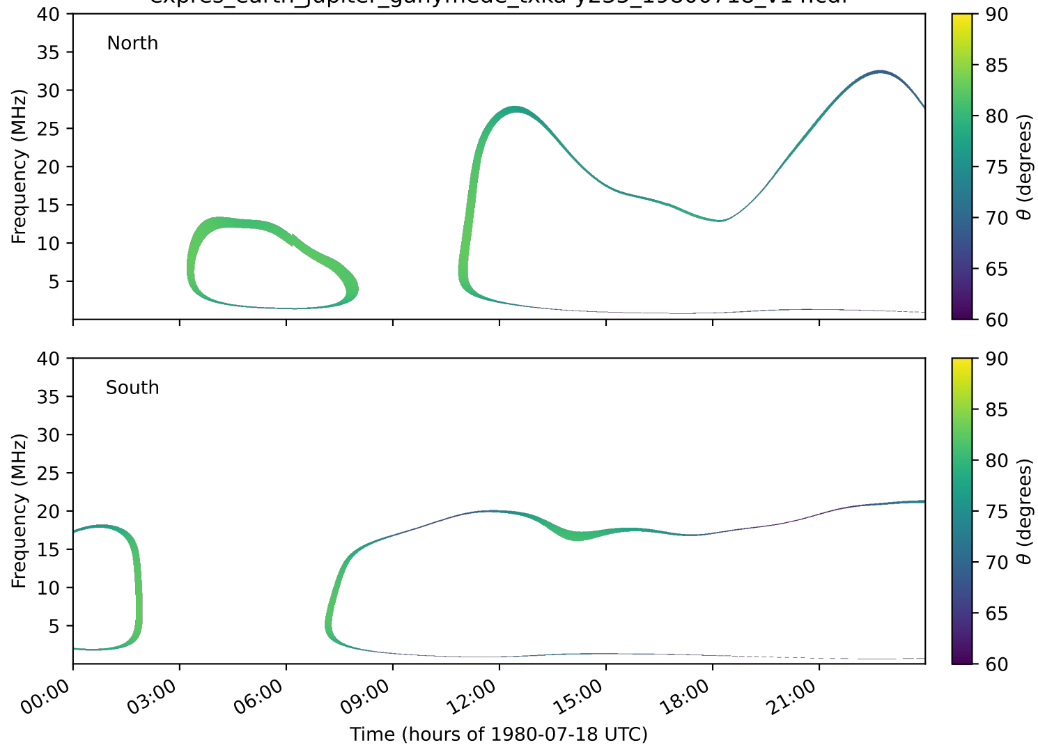
expres_earth_jupiter_ganymede_txka-y235_19800718_v14.cdf
