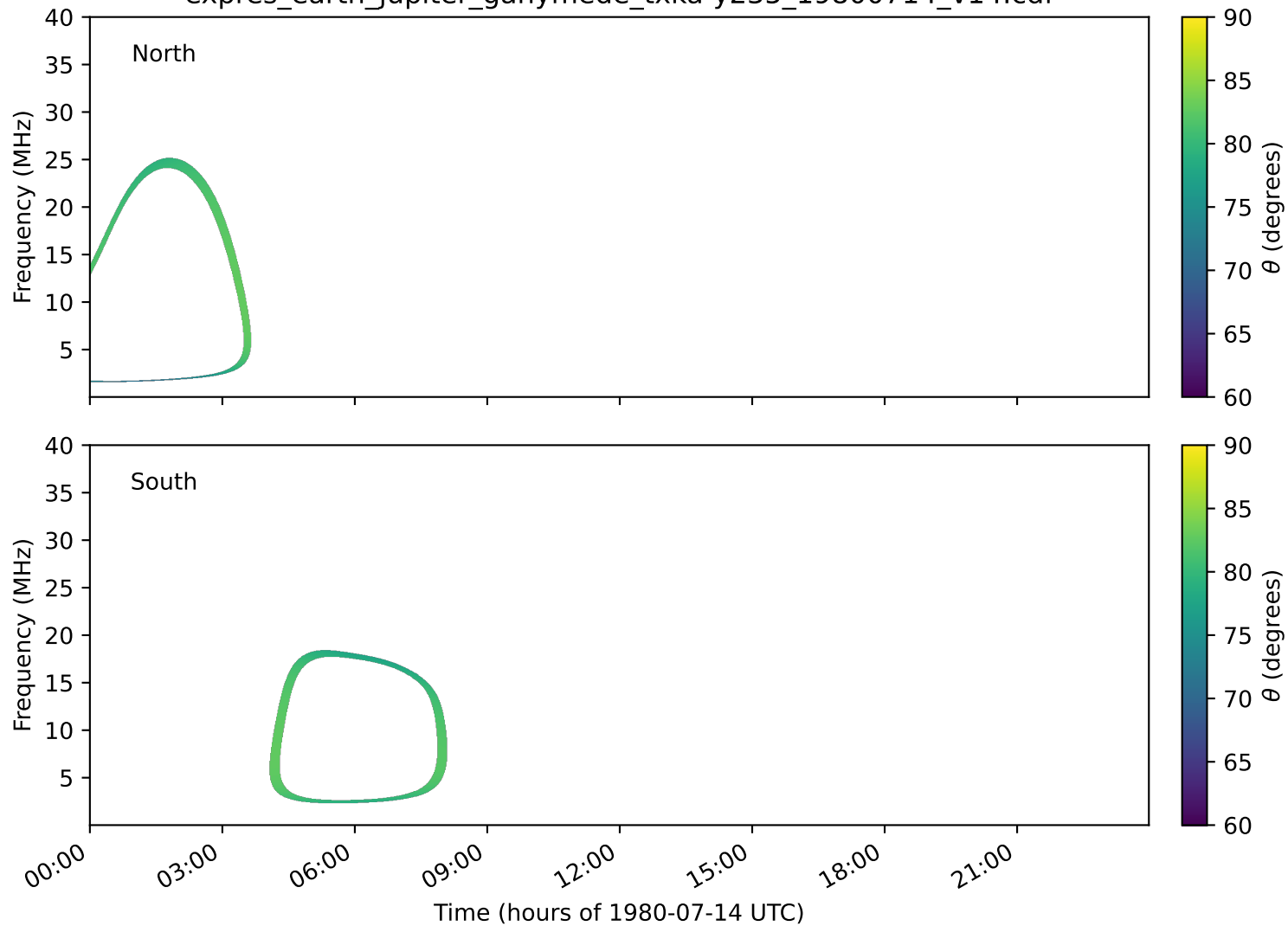
expres_earth_jupiter_ganymede_txka-y235_19800714_v14.cdf
