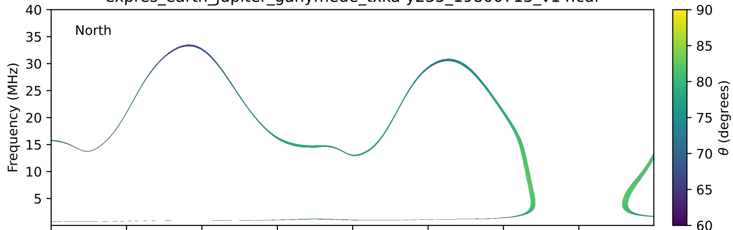
expres_earth_jupiter_ganymede_txka-y235_19800713_v14.cdf
