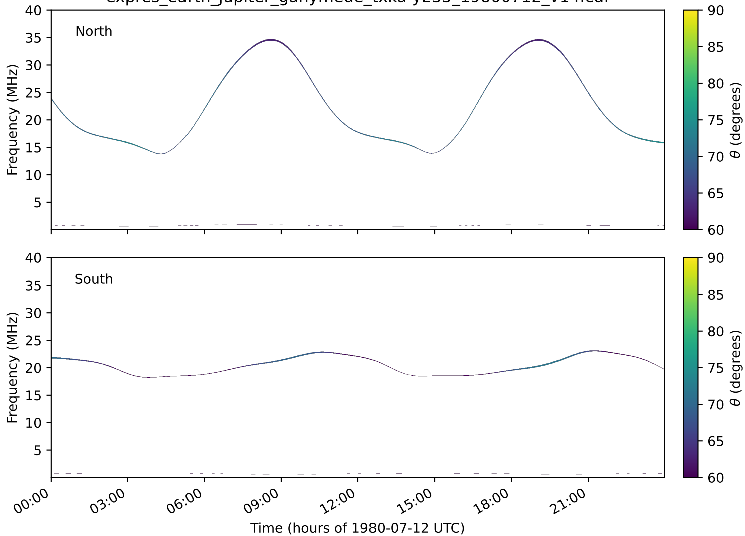
expres_earth_jupiter_ganymede_txka-y235_19800712_v14.cdf
