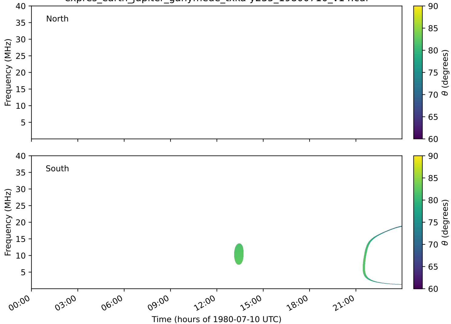
expres_earth_jupiter_ganymede_txka-y235_19800710_v14.cdf
