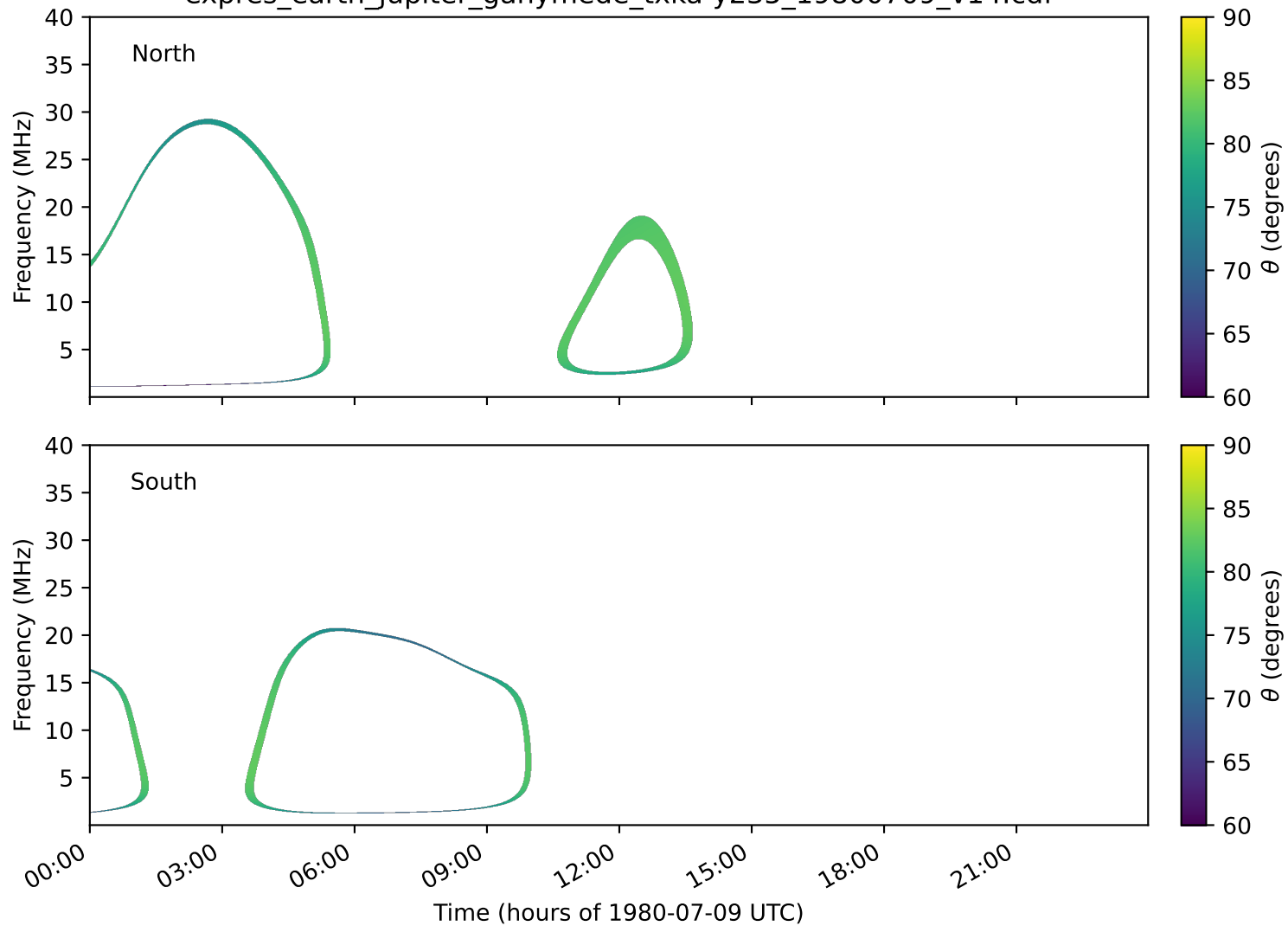
expres_earth_jupiter_ganymede_txka-y235_19800709_v14.cdf
