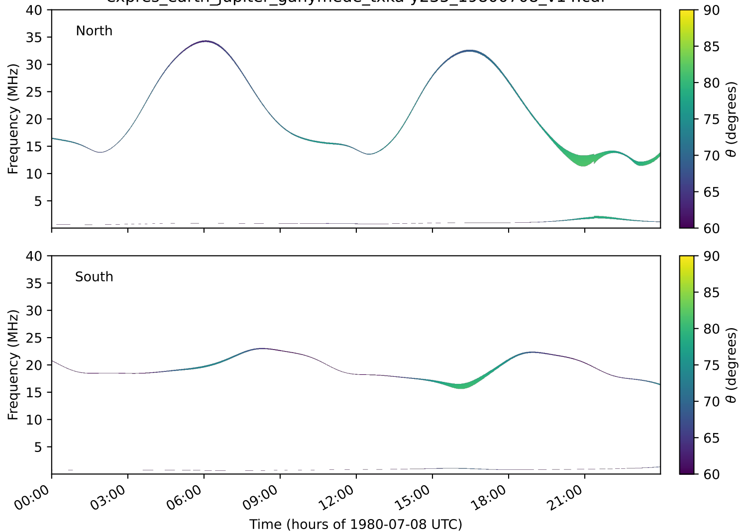
expres_earth_jupiter_ganymede_txka-y235_19800708_v14.cdf
