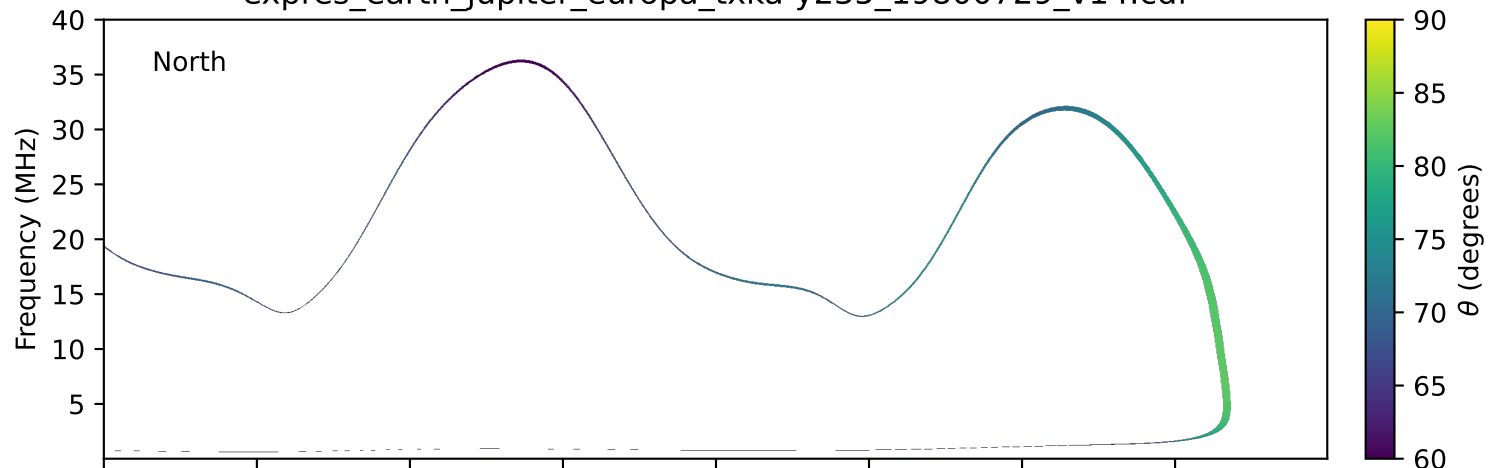
expres_earth_jupiter_europa_txka-y235_19800729_v14.cdf
