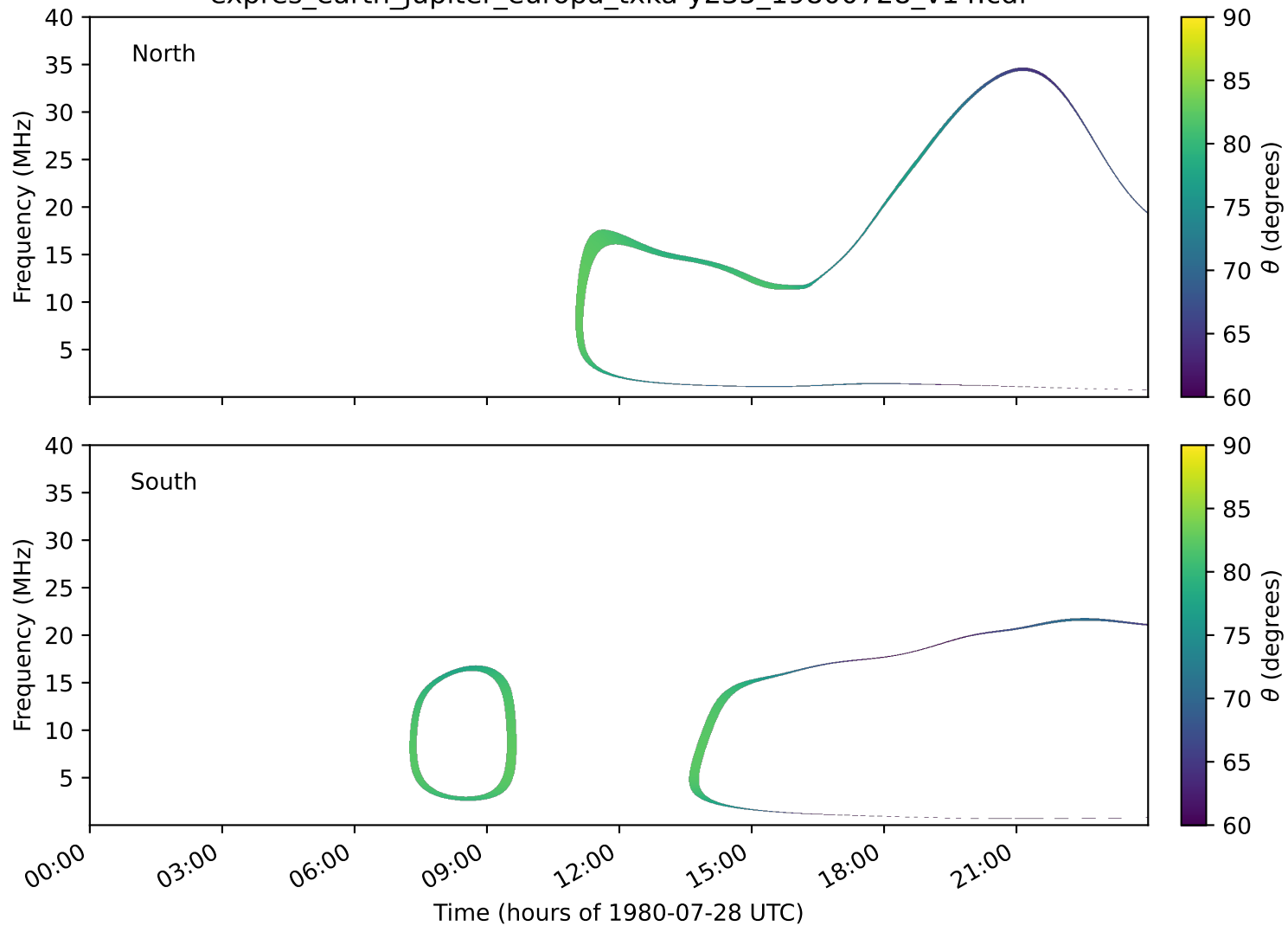
expres_earth_jupiter_europa_txka-y235_19800728_v14.cdf
