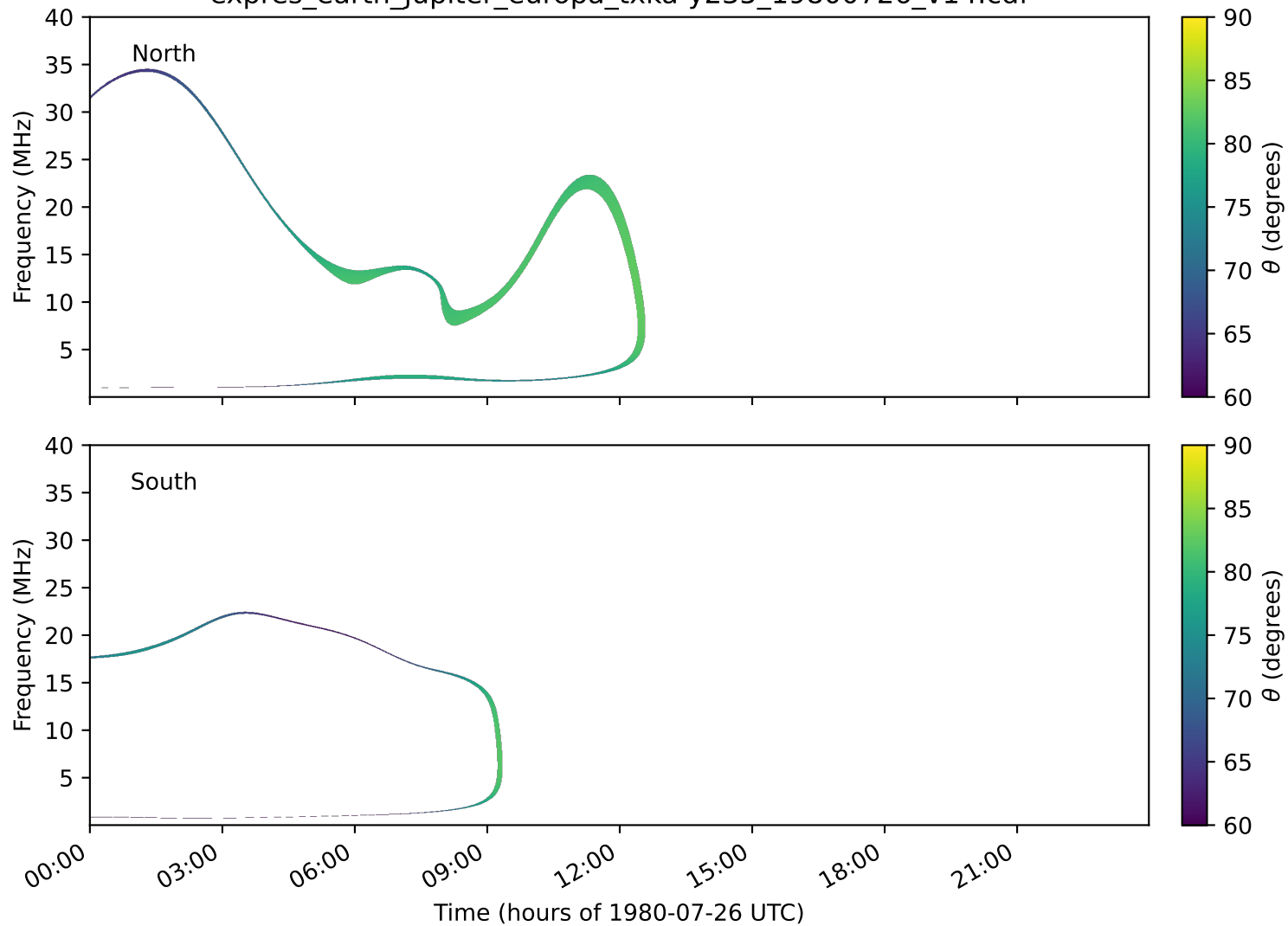
expres_earth_jupiter_europa_txka-y235_19800726_v14.cdf
