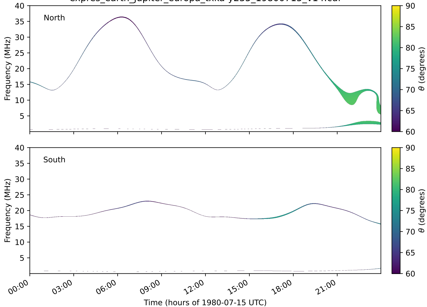
expres_earth_jupiter_europa_txka-y235_19800715_v14.cdf
