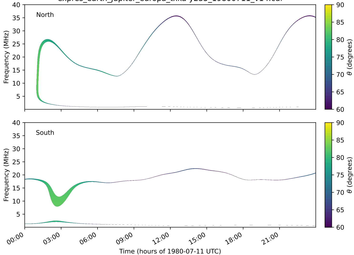
expres_earth_jupiter_europa_txka-y235_19800711_v14.cdf
