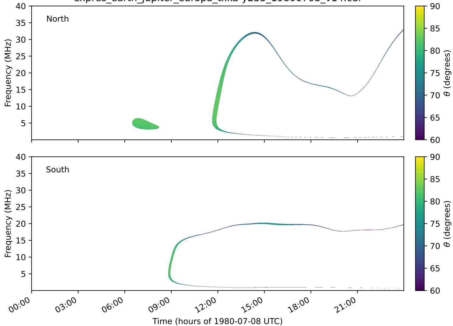
expres_earth_jupiter_europa_txka-y235_19800708_v14.cdf
