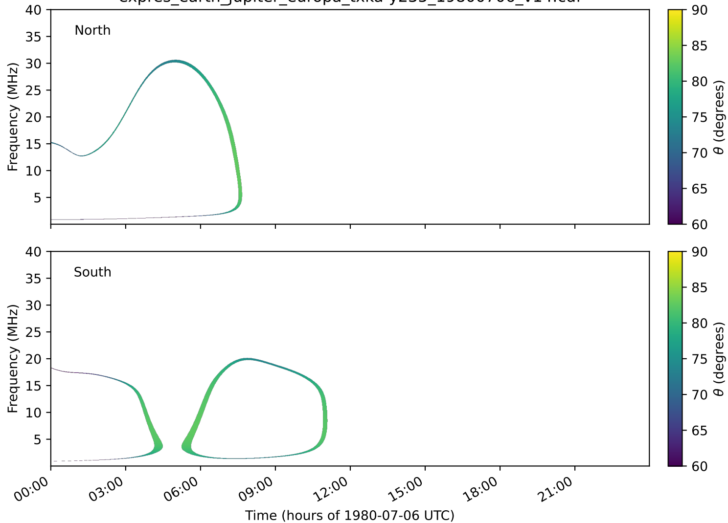
expres_earth_jupiter_europa_txka-y235_19800706_v14.cdf
