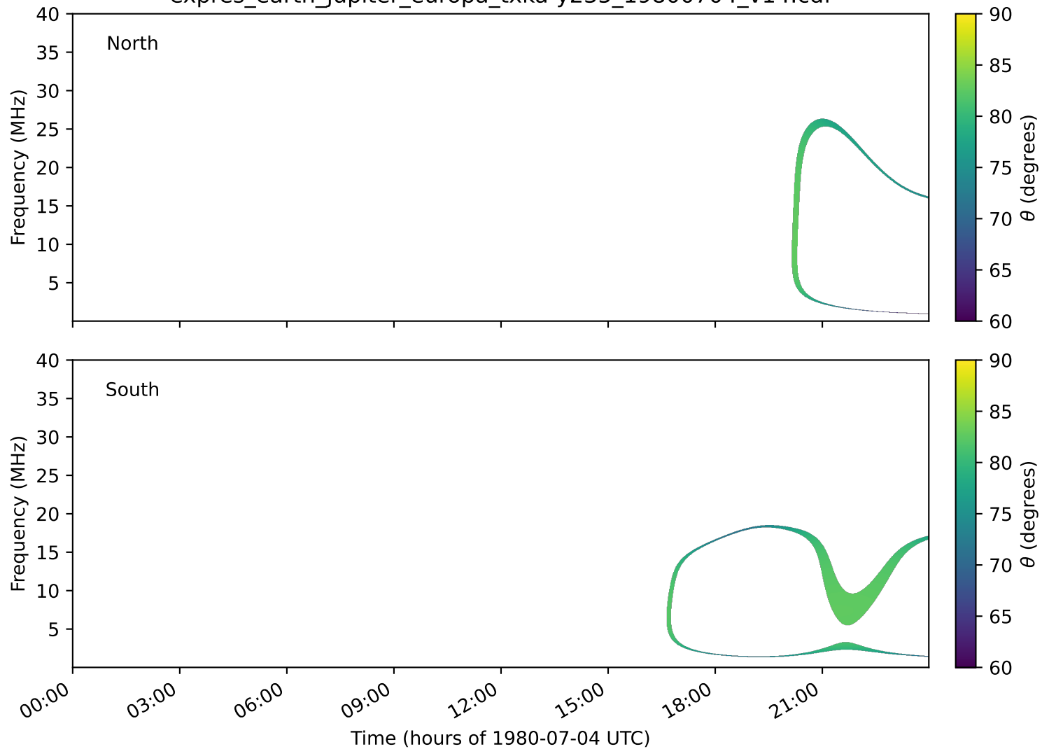
expres_earth_jupiter_europa_txka-y235_19800704_v14.cdf
