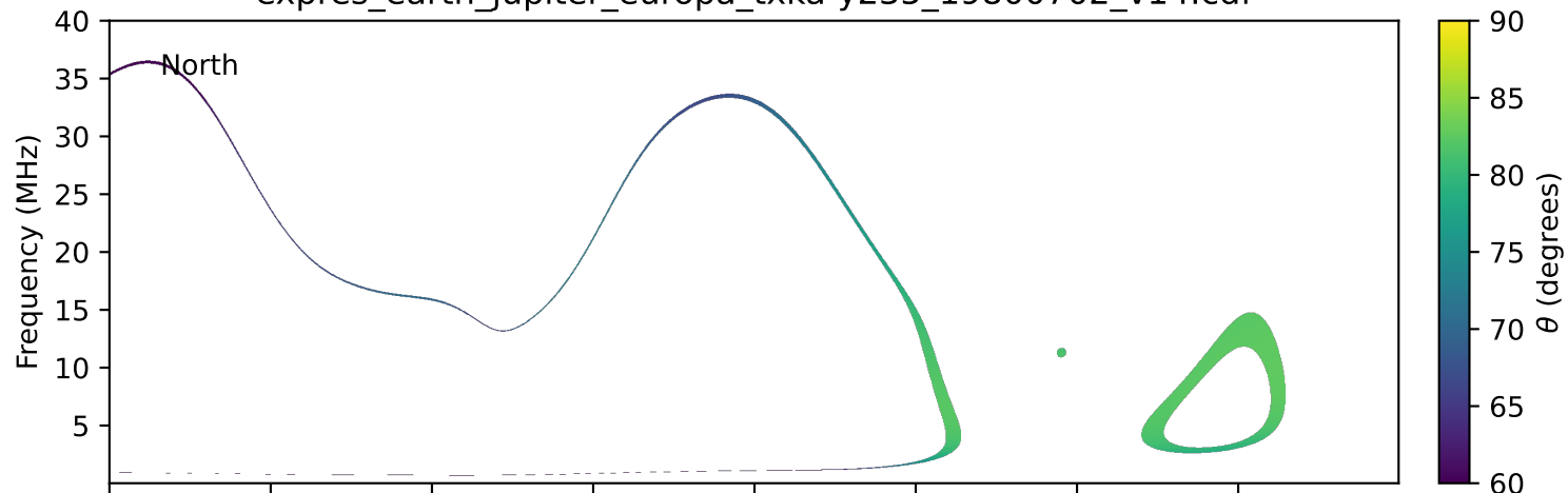
expres_earth_jupiter_europa_txka-y235_19800702_v14.cdf
